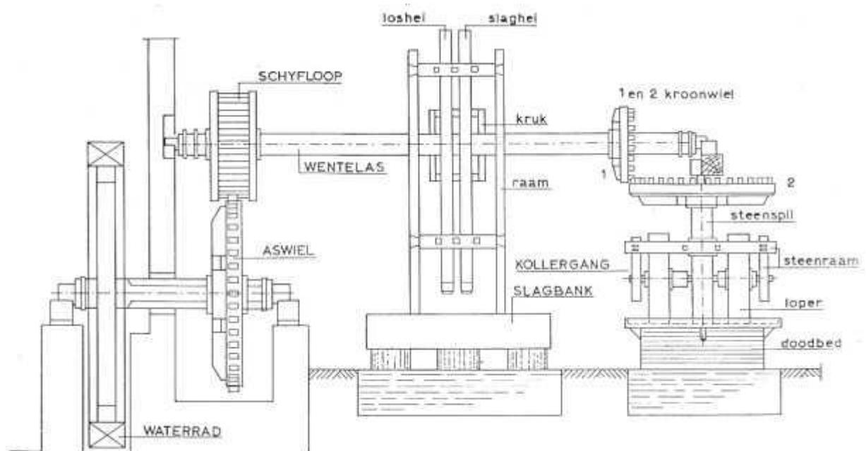
The gearing in an oilmill.
