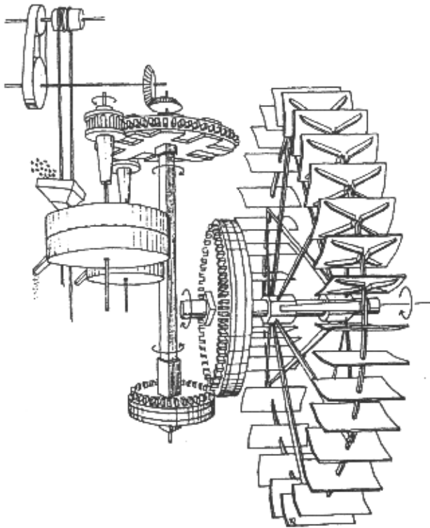
The gearing in the corn mill.
