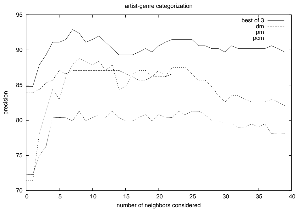
Fig. 4. Precision (%) for classification.
