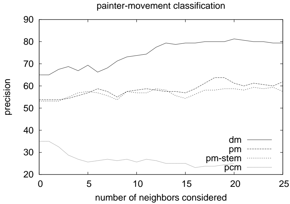
Fig. 1. Precision (%) for classification.
