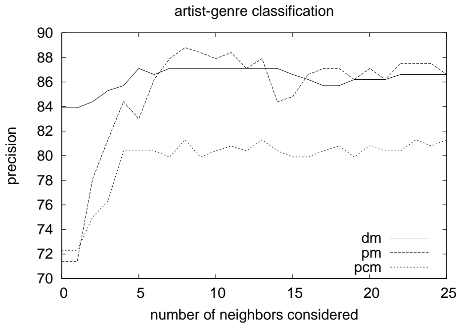
Fig. 2. Precision (%) for classification.
