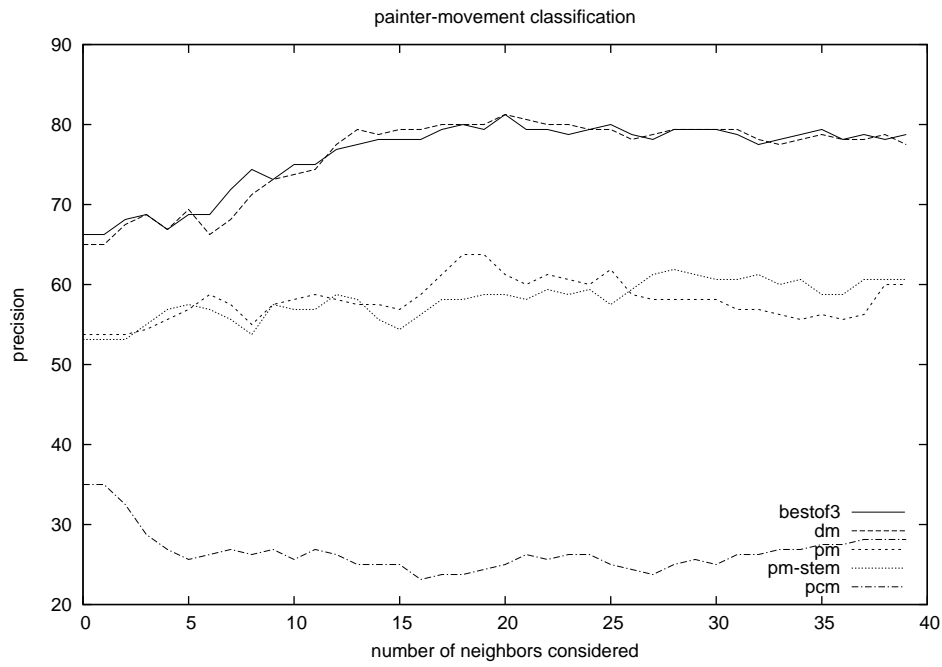
Fig. 3. Precision (%) for classification.
